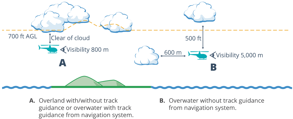
Figure 5: VMC criteria for rotorcraft in Class G noncontrolled airspace (MOS Table 2.07)
