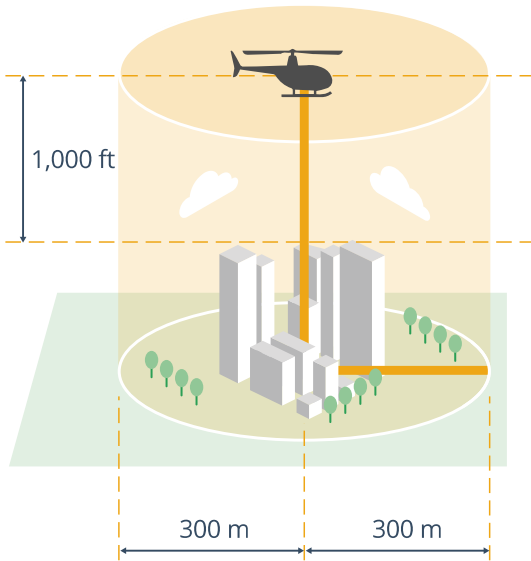
Figure 20: Minimum height populous areas and public gatherings for rotorcraft
