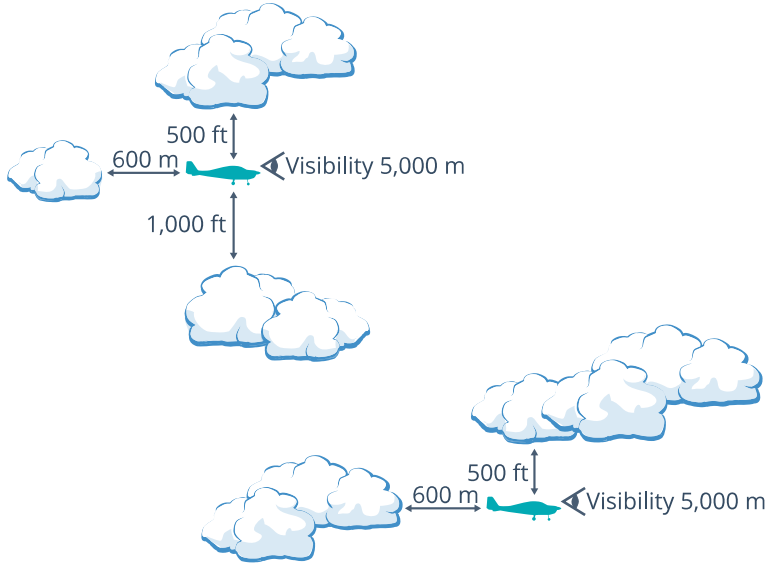
Figure 4: VMC criteria all aircraft for Class D controlled airspace (MOS Table 2.07)
