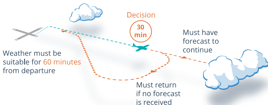
Figure 12: Departure aerodrome return decision
