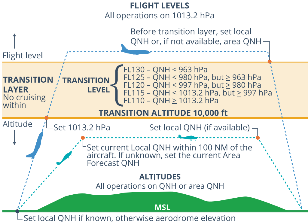
Figure 16: Positions to change between QNH and 1013.2 hPa
