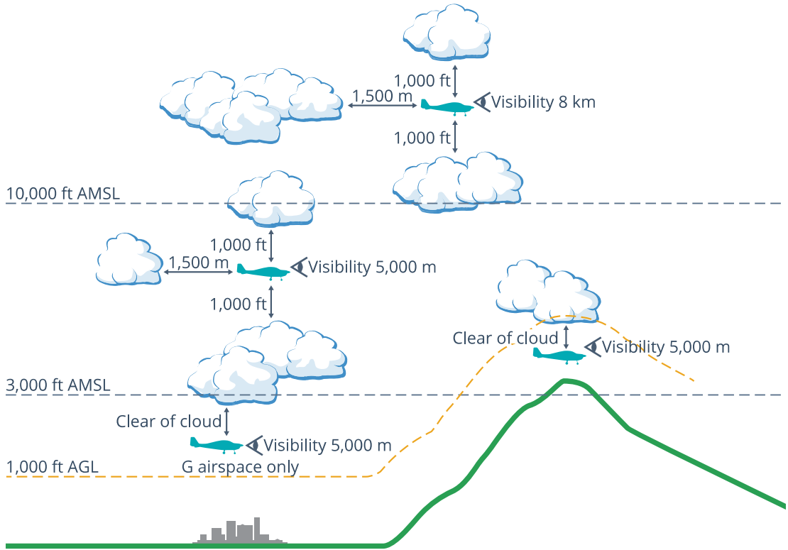
Figure 3: VMC criteria all aircraft Class A, B, C, E and G (MOS Table 2.07)
